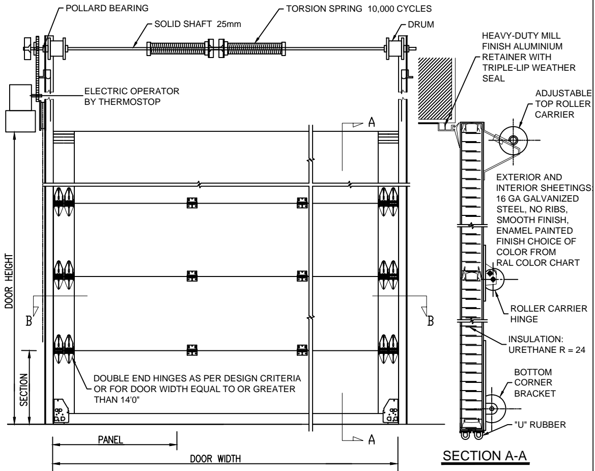
INTERIOR ELEVATION
